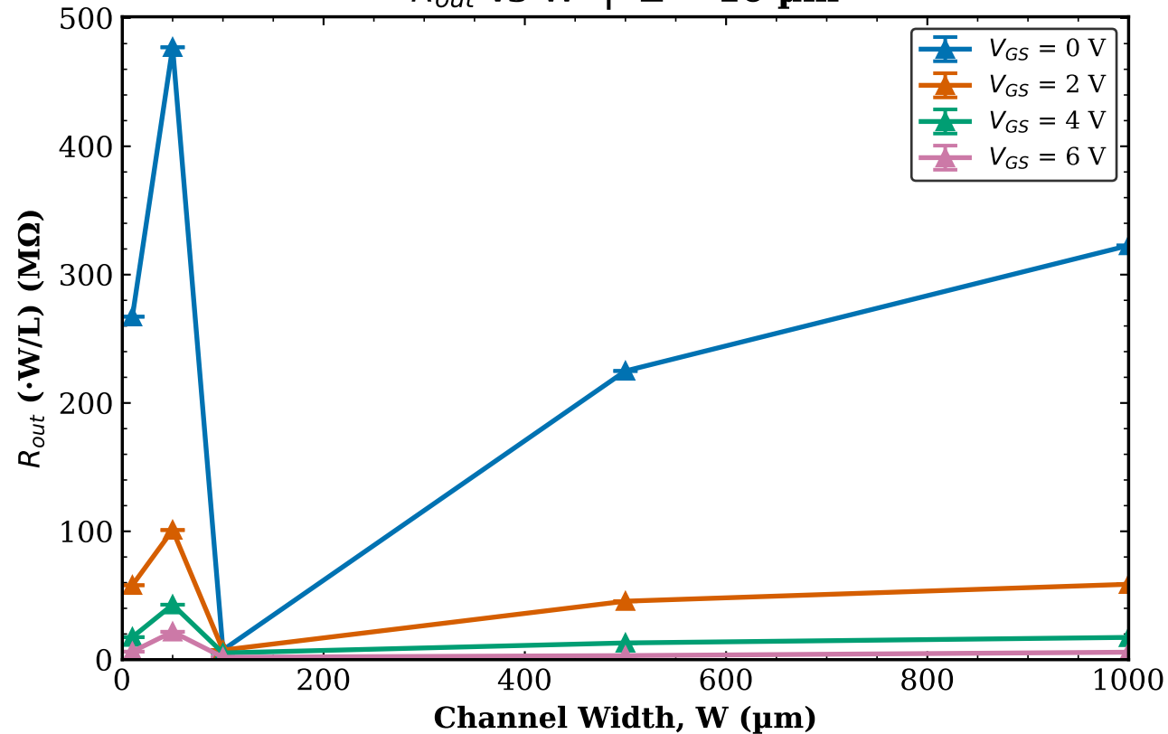
TFT1 Transistor 2 R_{out} vs W | L = 10\text{ }\mu\text{m}
